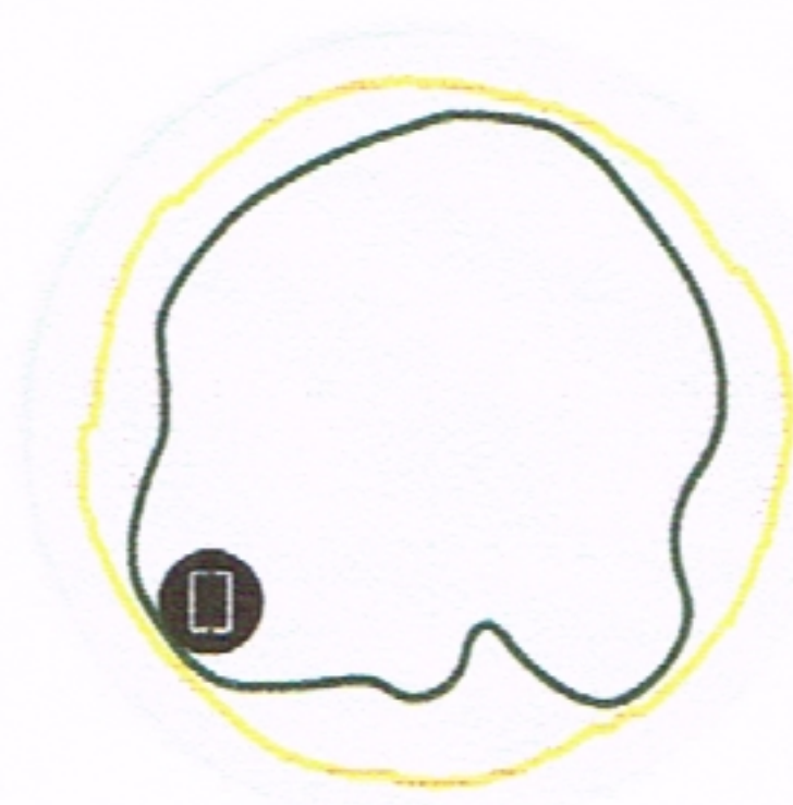
Figure 2 - T310d 2.4GHz Azimuth Antenna Patterns
