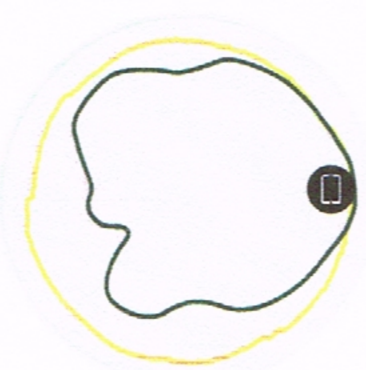
Figure 3 - T310d 5GHz Azimuth Antenna Patterns
